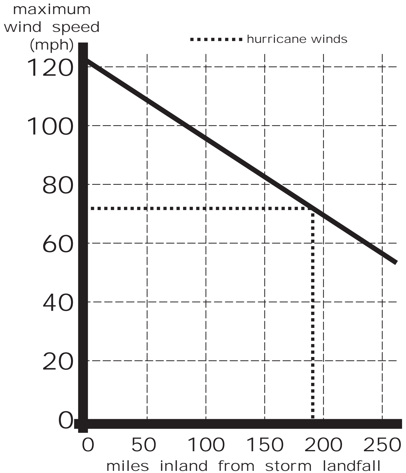
Figure 9: Estimated maximum wind speed at various distances inland from a category 3 hurricane landfall. (NOAA data)
