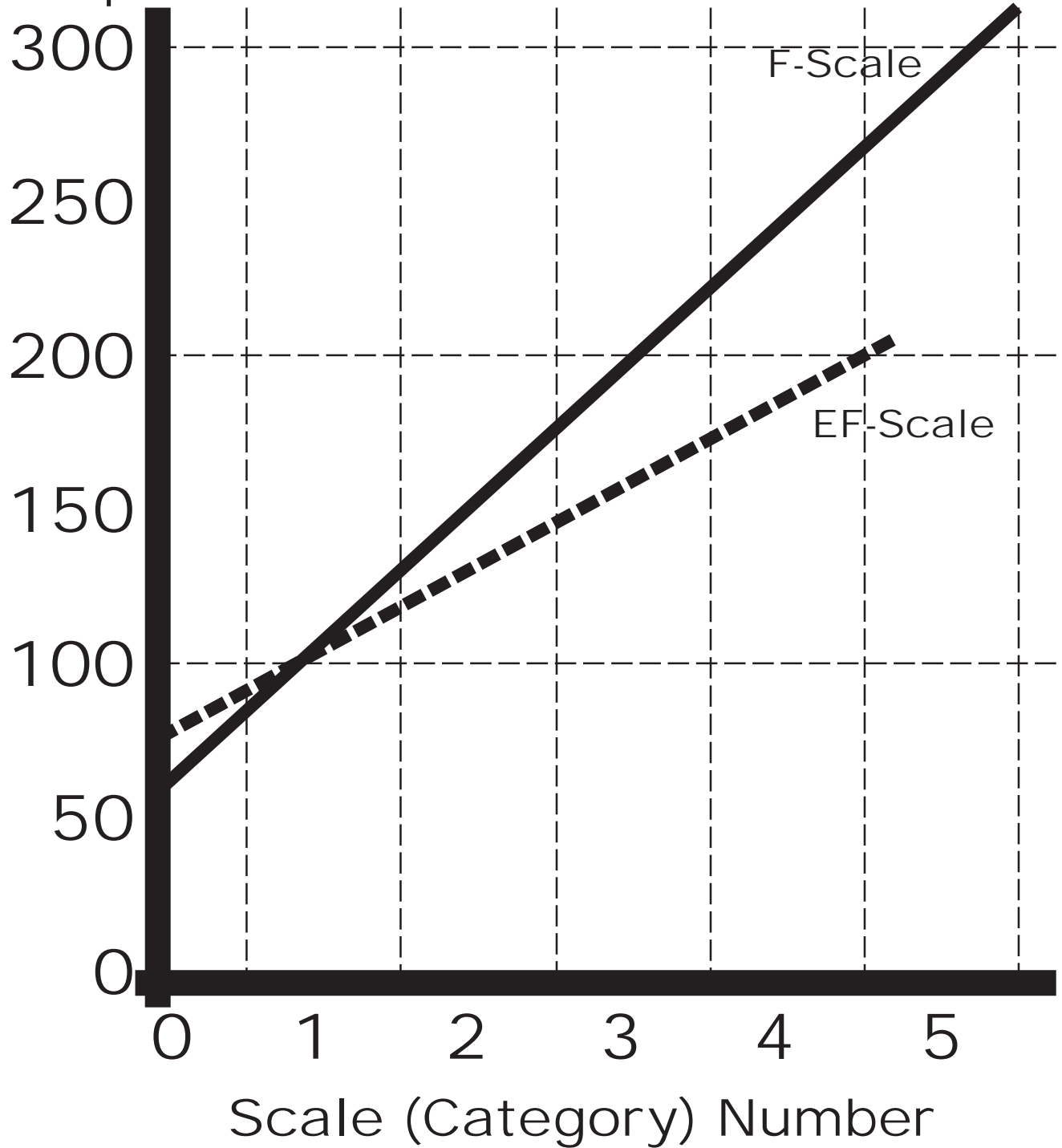
Figure 15: Comparison of F-Scale (solid line) and EF-Scale (dotted line) values. Note both scales are curves but are shown here as straight lines.
