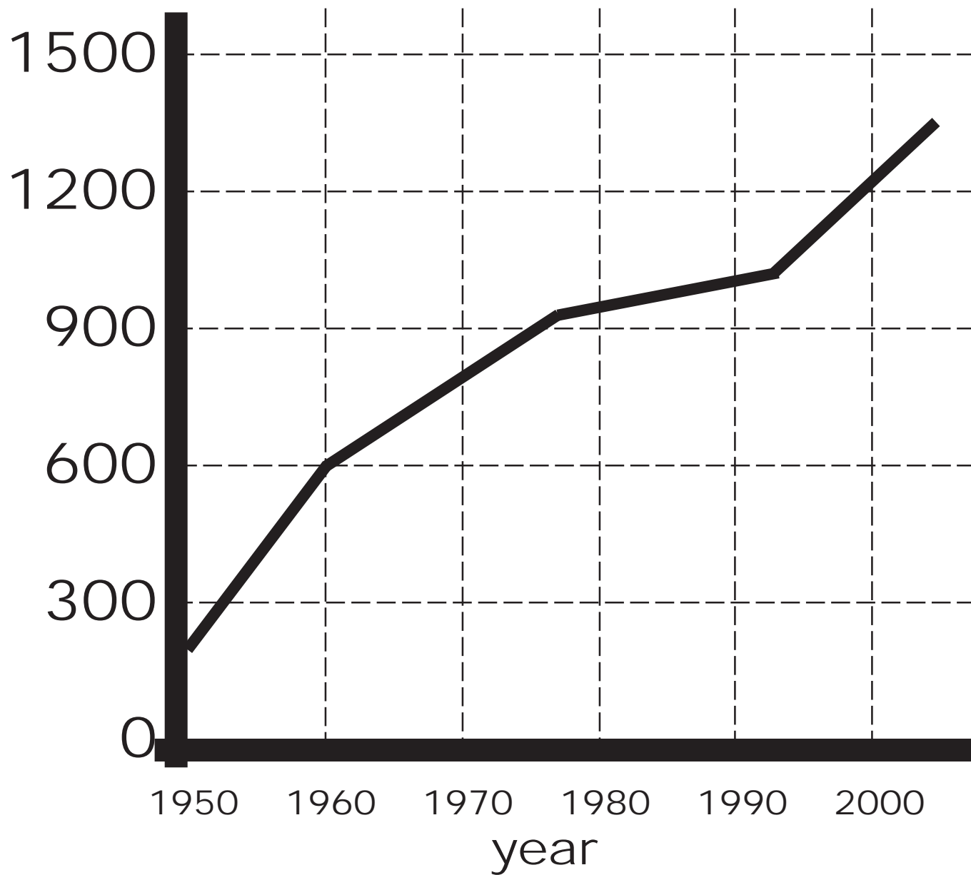
Figure 11: General trend line for tornado numbers. (NOAA data)
